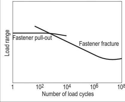
Effect of number of cycles on failure mode DX fastener in steel (correctly placed)
