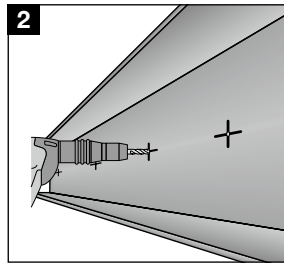
2 Pre-drill with TX-BT 4/7 step shank drill bit.
