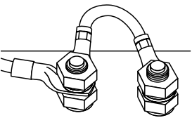
Double-point connection
