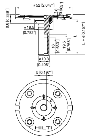
X-FCM-R grating disc
