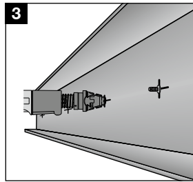
3 Drive fastener only with DX 351 BT tool and 6.8/M brown cartridge.
