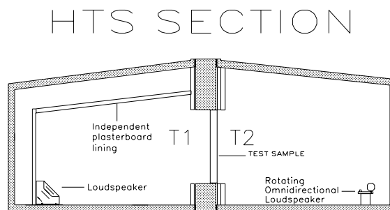
Figure 3. Chamber layout.
