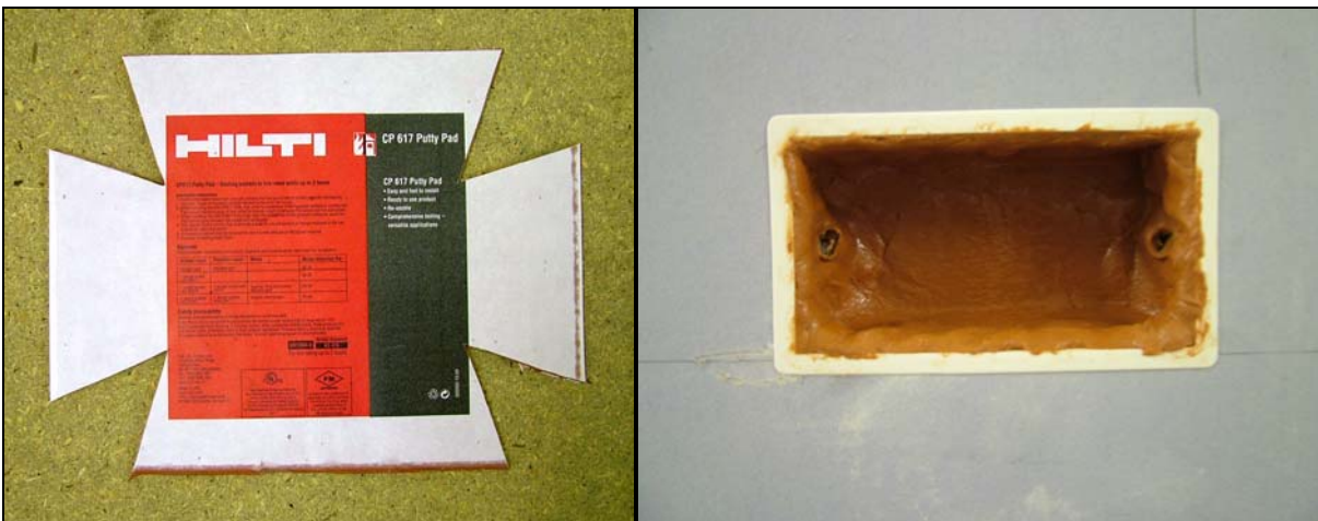
Photograph 3. Hilti Putty Pad cut to locate within wall box Photograph 4. Hilti Putty Pad fitted into wall box
