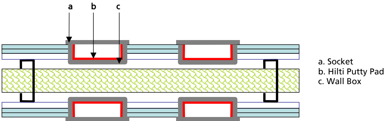
Figure 2. Partition as in figure 1 with wall boxes, sockets and Hilti Putty Pads installed.
