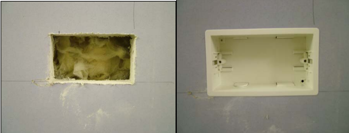
Photograph 1. Hole created for wall box Photograph 2. Wall box fitted into partition
